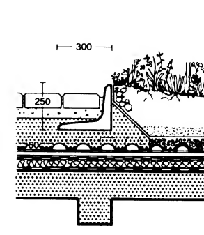
⑮ Transition from road surface to intensive roof cultivation
